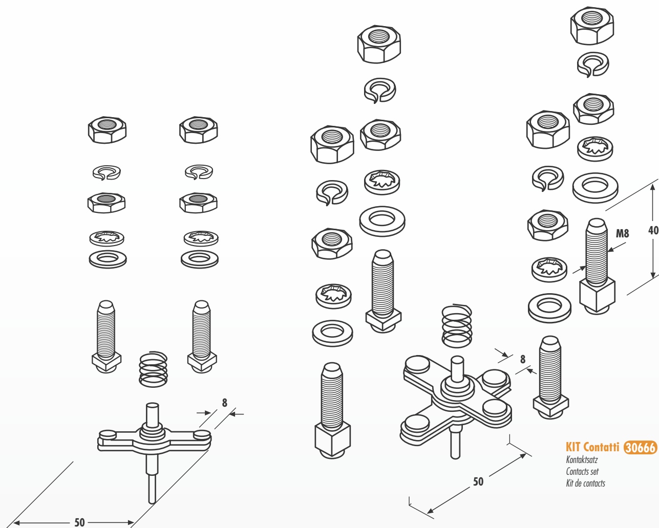
KIT Contatti 30665 Kontaktsatz Contacts set Kit de contacts
